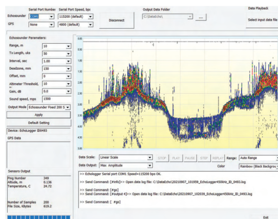
Custom User Interface with Real-Time Sonar Echogram
